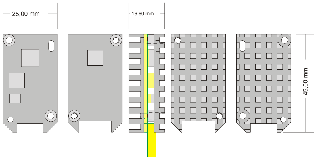
Antminer U1 advanced Heatsink, Material: 8mm Aluminium
