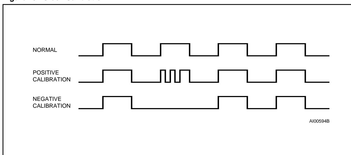
Figure 10. Clock Calibration
