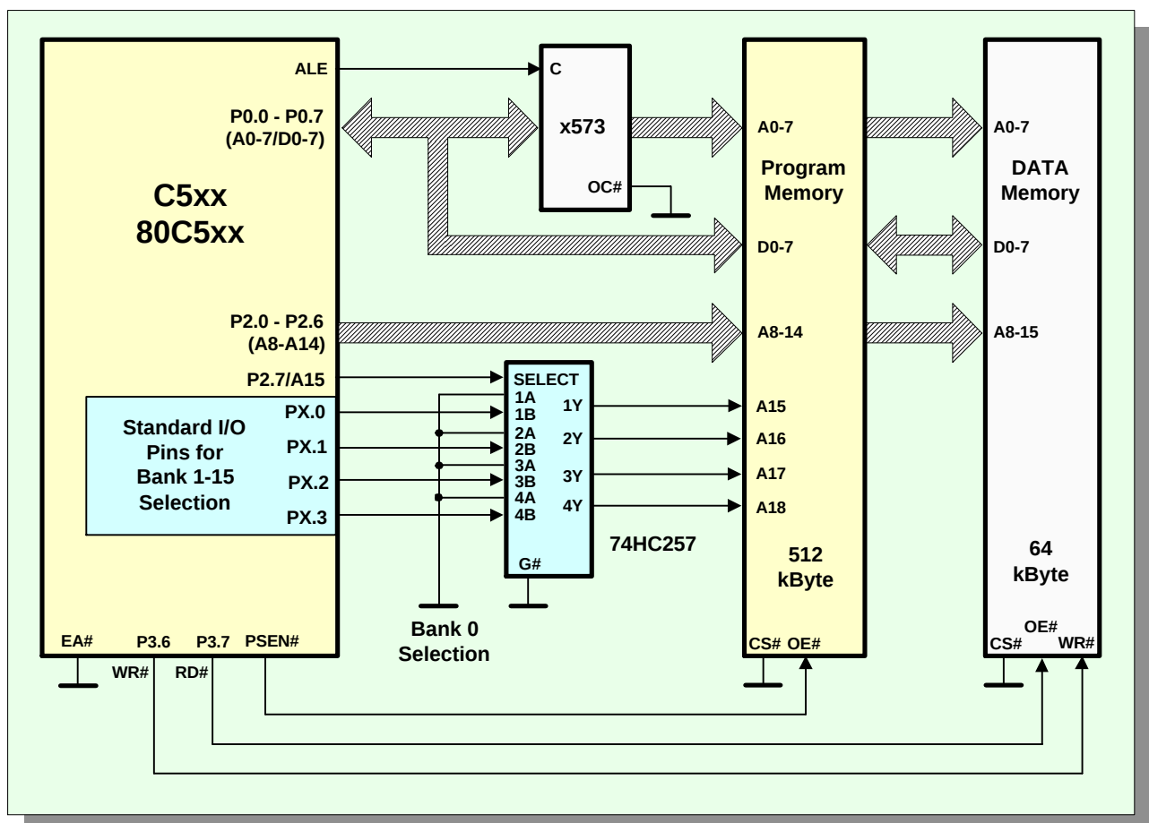
Figure 3: Schematic for External Memory Bus Interface
