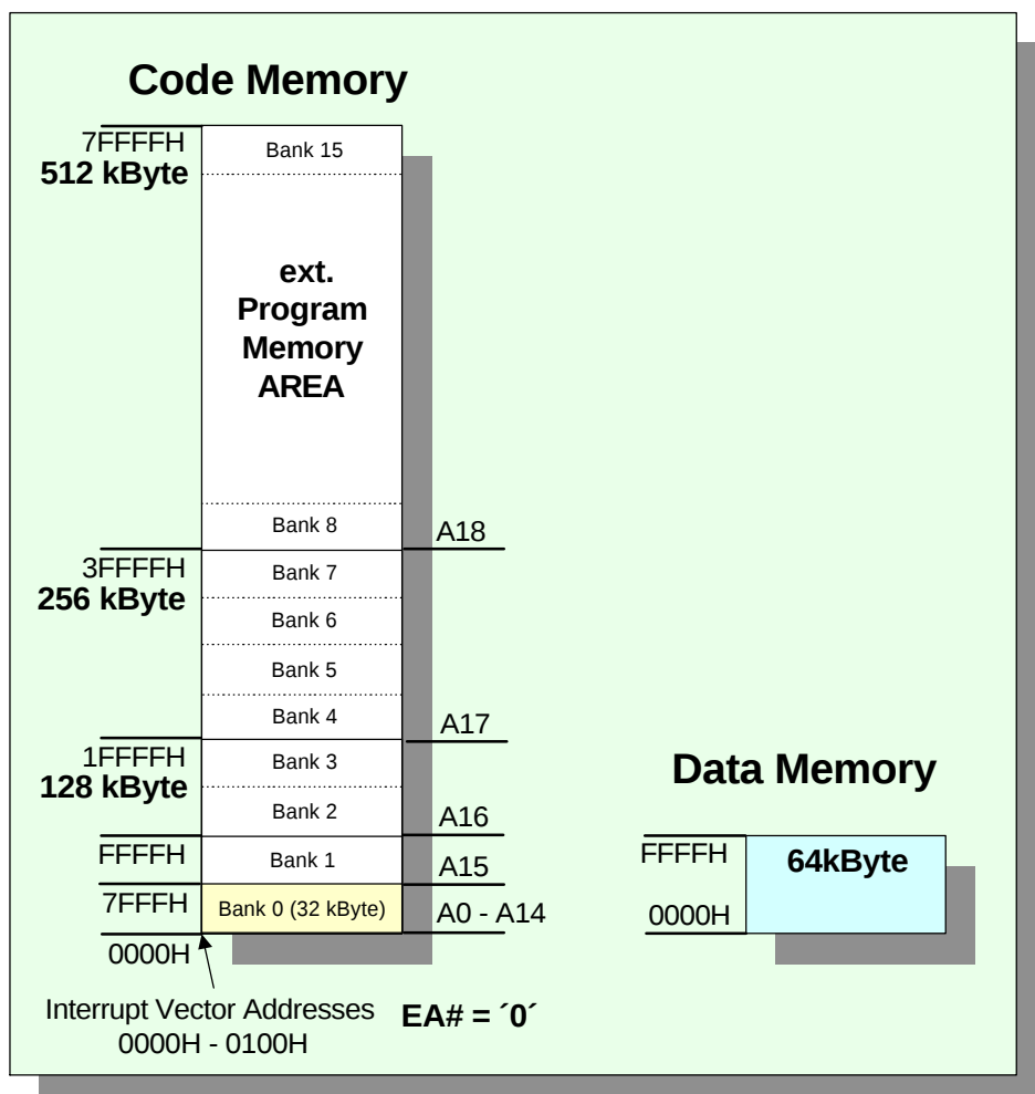
Figure 2: External Memory Organization in 'Expanded Configuration'
