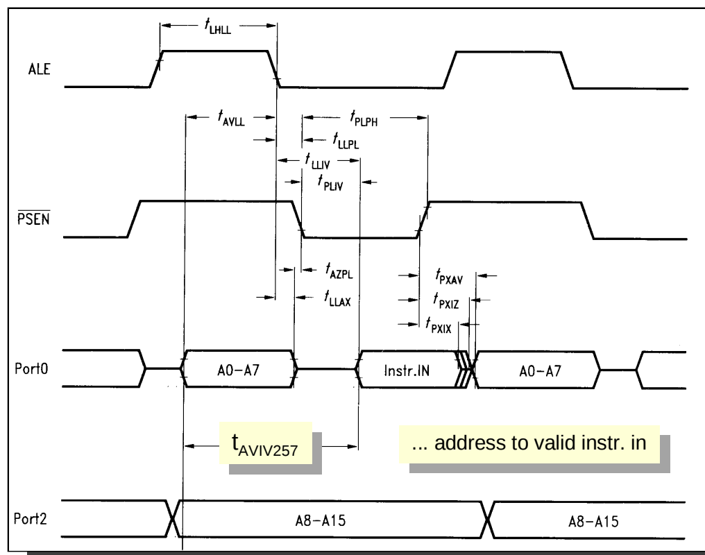
Figure 4: Program Memory Read Cycle
