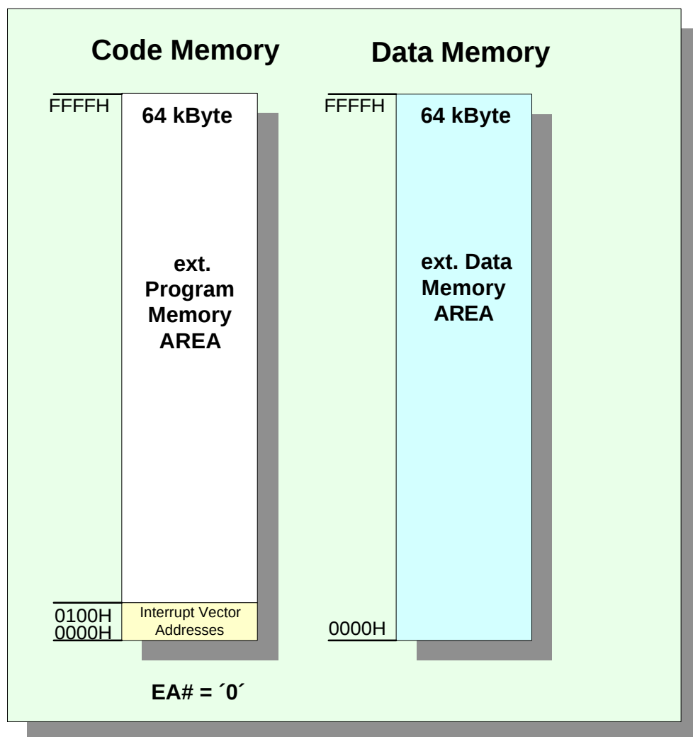
Figure 1: External Memory Organization in 'Normal Configuration'
