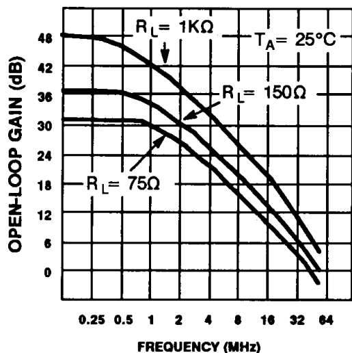
OPEN-LOOP GAIN vs. FREQUENCY
