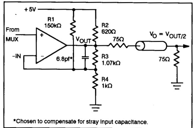
Figure 5. Minimizing Phase Distortion
