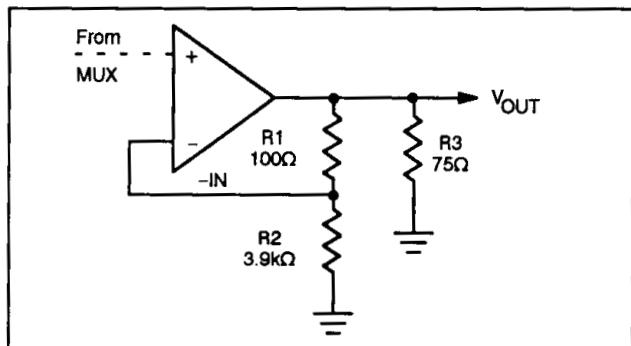
Figure 2. Unity-Gain Connections
