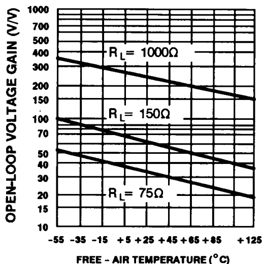
OPEN-LOOP GAIN vs. TEMPERATURE
