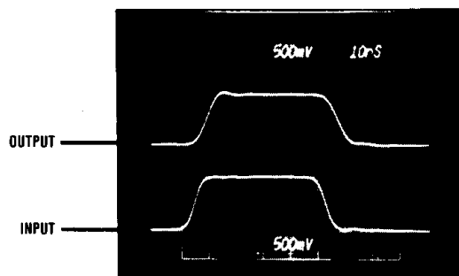
MAX455 PULSE RESPONSE
