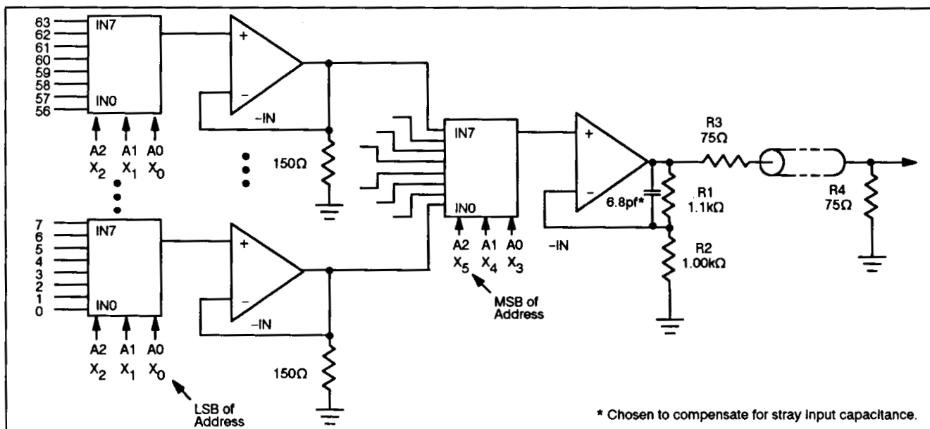
Figure 3. Nine MAX455s Used to Multiplex 64 Channels.
