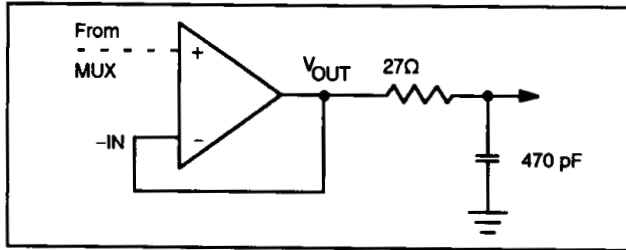
Figure 4. Isolating a Large Capacitive Load.
